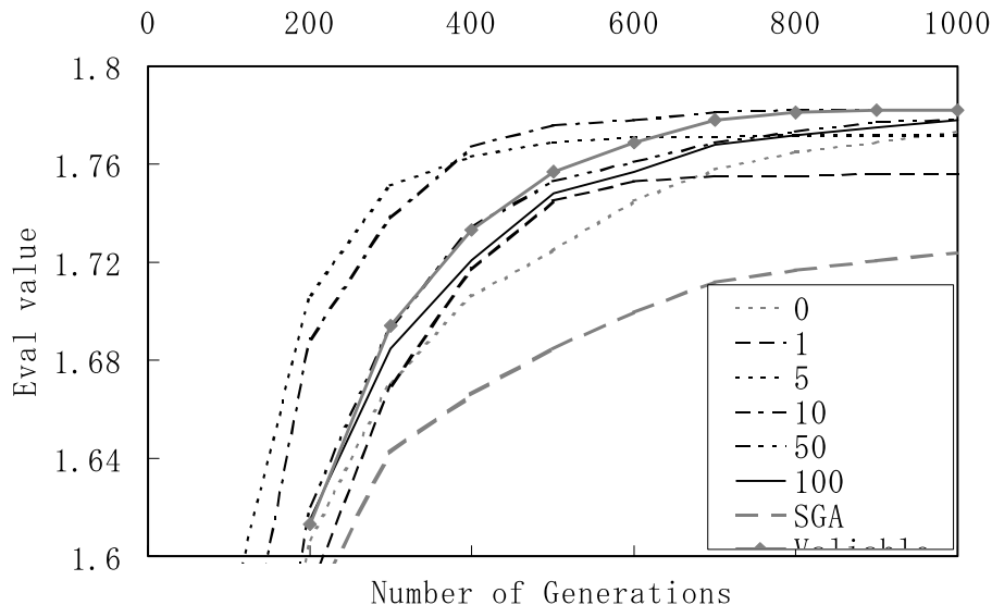
Fig. 2. Effect of Migration Interval on the fitness history.
