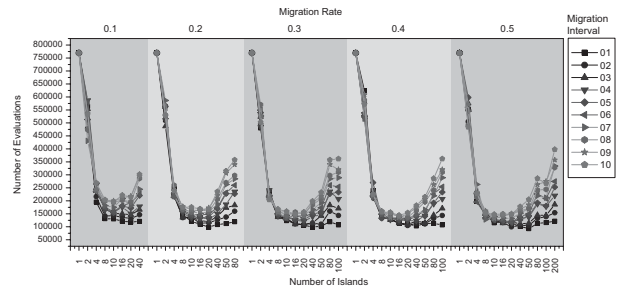
⊠ 9: Migration Interval, Migration Rate, Number of Islands (Schwefel)
