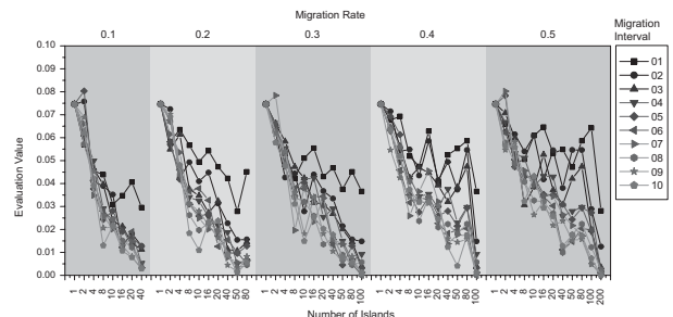
⊠ 10: Migration Interval, Migration Rate, Number of Islands (Ridge)
