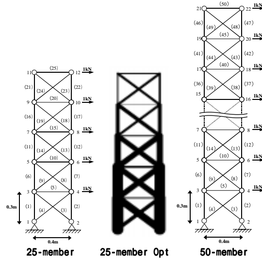
図 3: Truss structure
