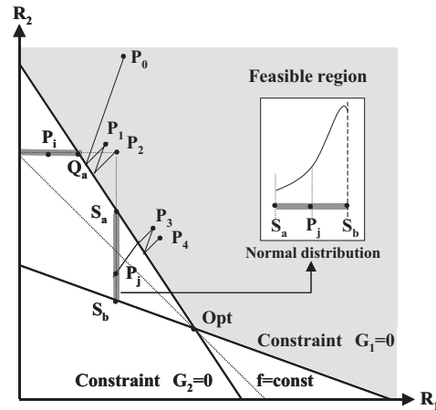
図 1: The way of generating a new point
